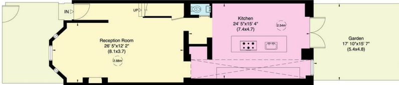
Ground Floor
